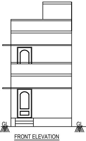
FRONT ELEVATION
