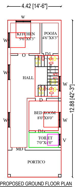
PROPOSED GROUND FLOOR PLAN
