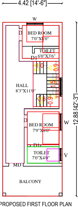
PROPOSED FIRST FLOOR PLAN
