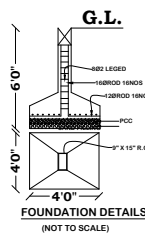
EARTHQUAKE SAFE DESIGN (NOT TO SCALE)
