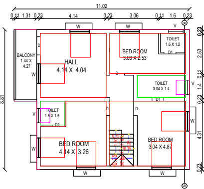
PROPOSED FIRST FLOOR BUILDING
