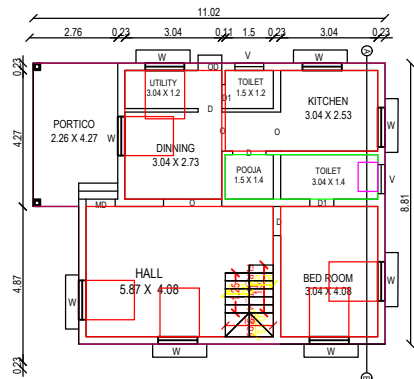
PRO. GROUND FLOOR BUILDING
