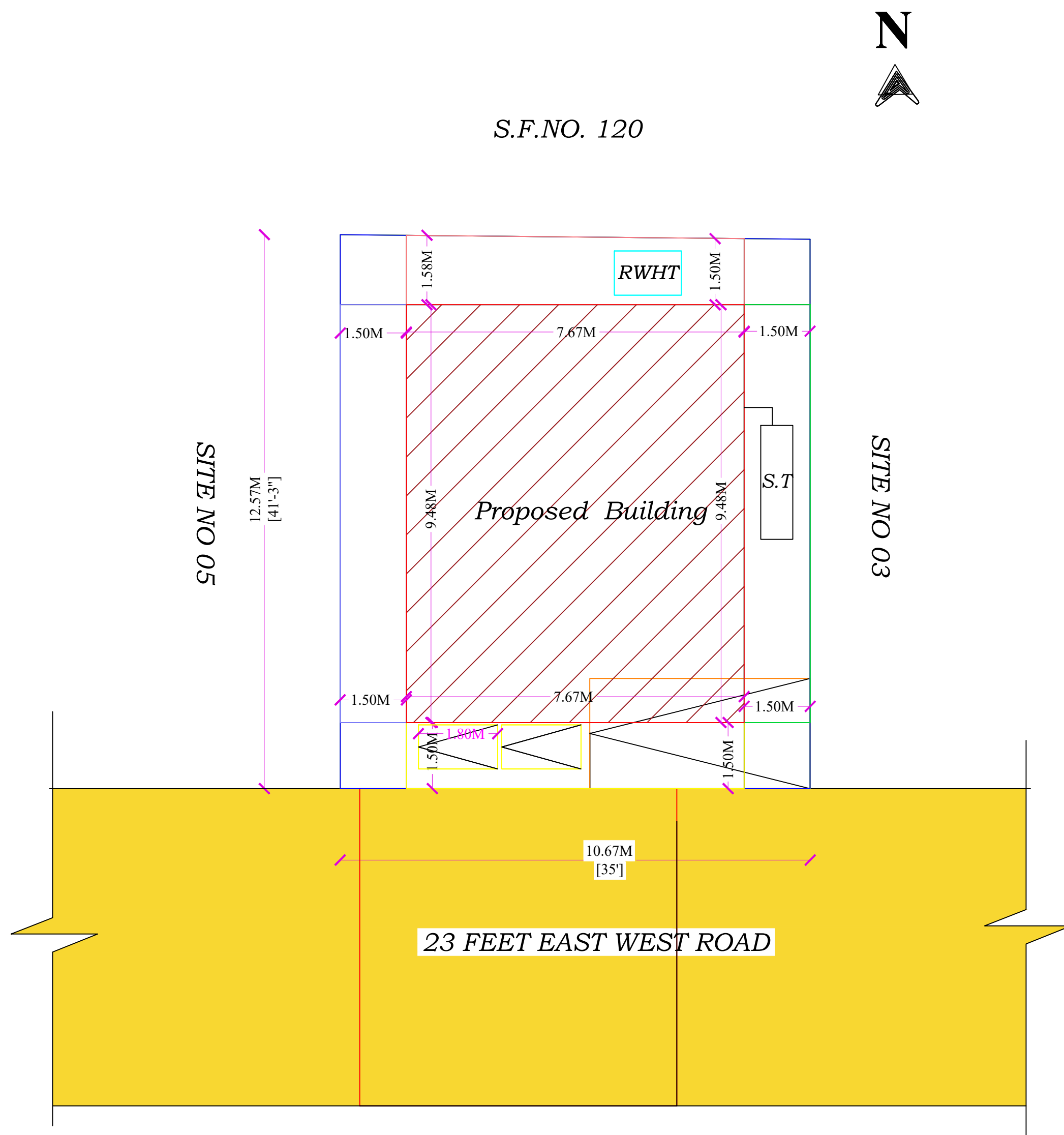
Site Plan (Scale 1"=8'0") SITE PLAN
