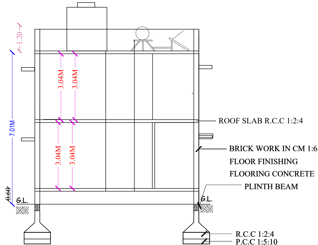
SECTION "A-A"
