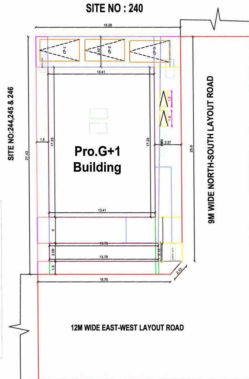
SITE PLAN (SCALE 1" : 8' 0")
