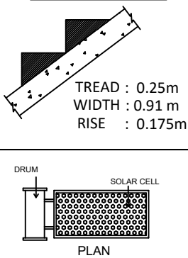
PLAN
