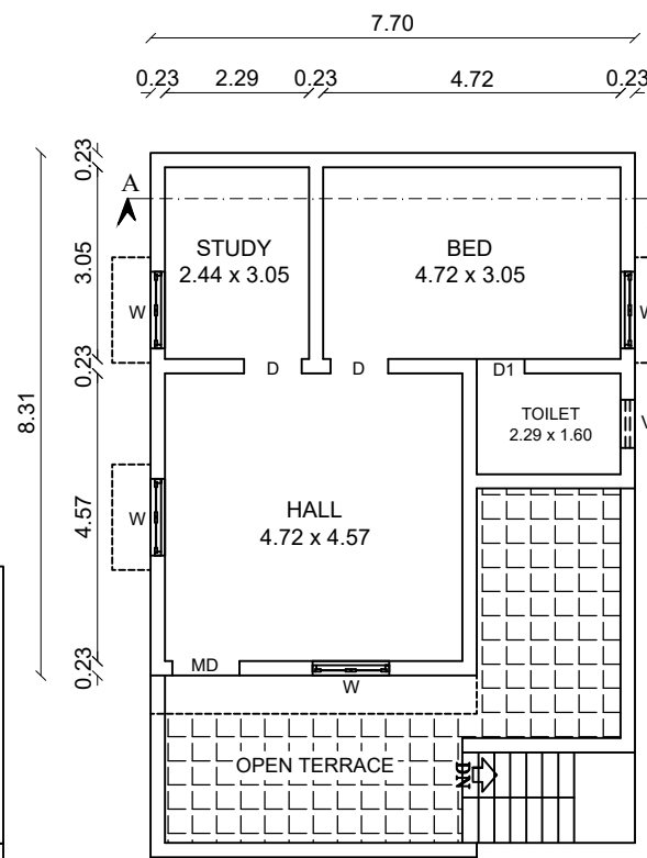
PRO. ADDL. FIRST FLOOR PLAN
