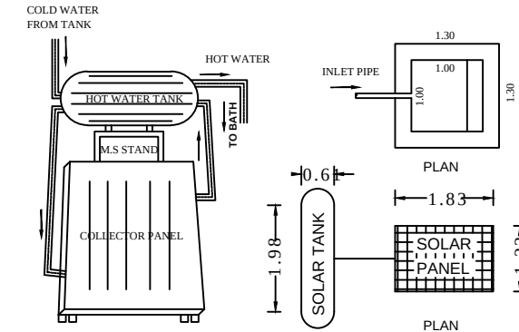
SOLAR WATER HEATER SYSTEM
