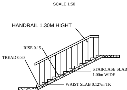
STAIRCASE DETAILS
