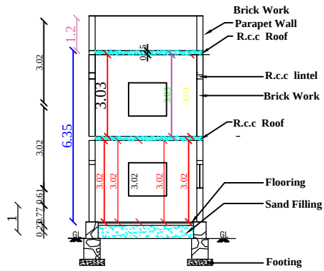
SECTION AB
