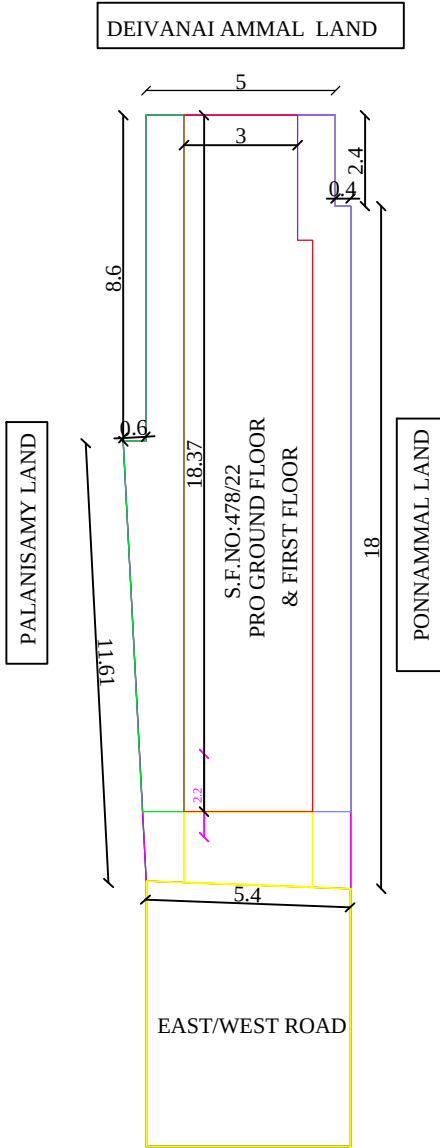
SITE PLAN
