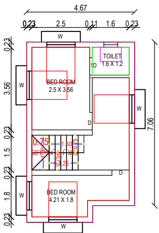
PROPOSED FIRST FLOOR BUILDING
