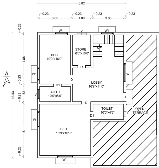
Proposed First Floor Plan FLOOR01
