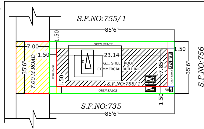
SUPER IMPOSED SITE PLAN
