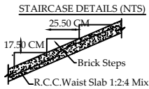
STAIRCASE DETAILS (NTS)
