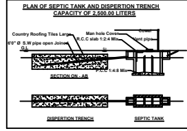
PLAN OF SEPTIC TANK AND DISPERSION TRENCH
