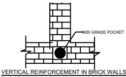
VERTICAL REINFORCEMENT IN BRICK WALLS
