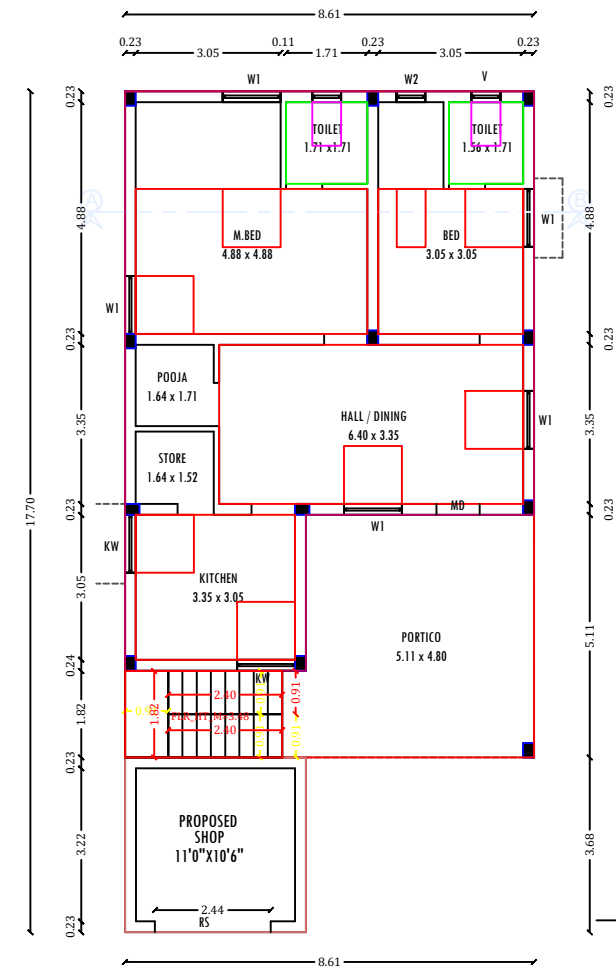
ADDITIONAL GROUND FLOOR PLAN
