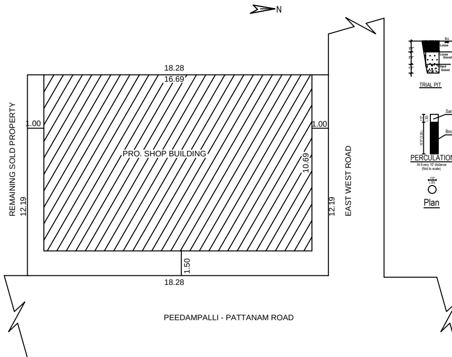
SITE PLAN
