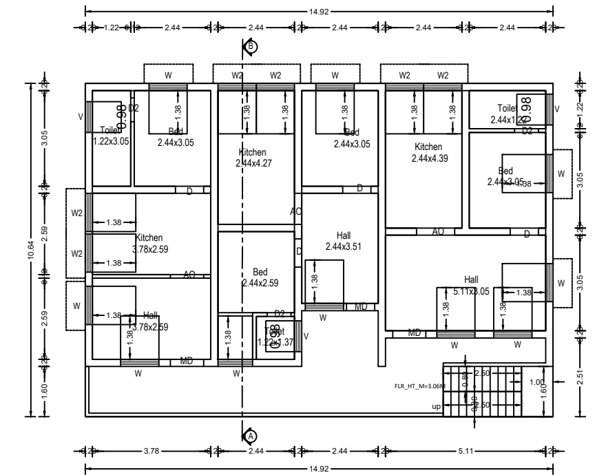
Plan Scale 1:100 First floor
