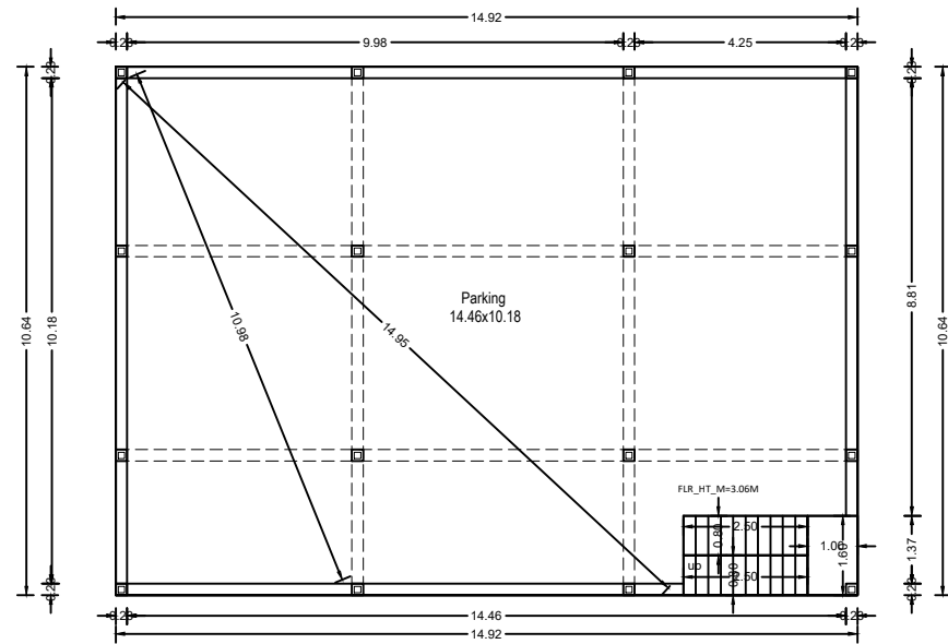
Stilt Floor Scale 1:100
