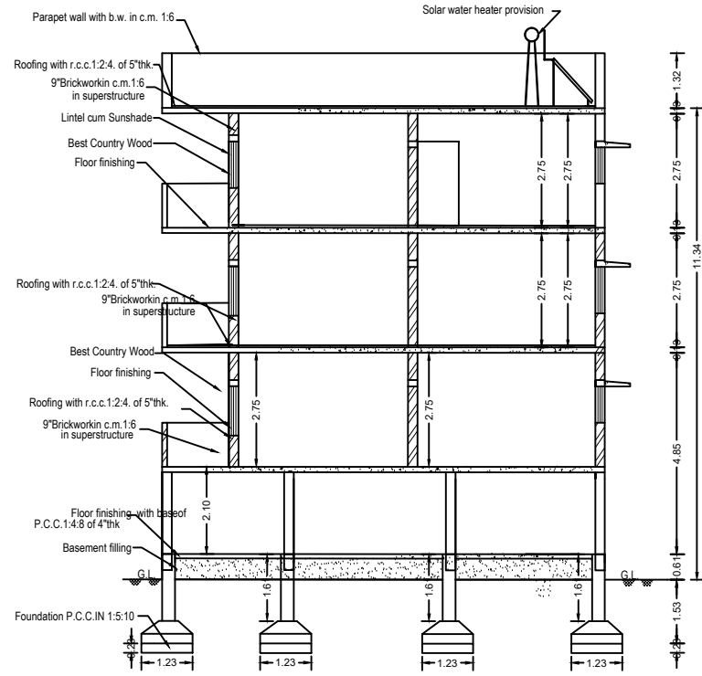
Section "AB"
