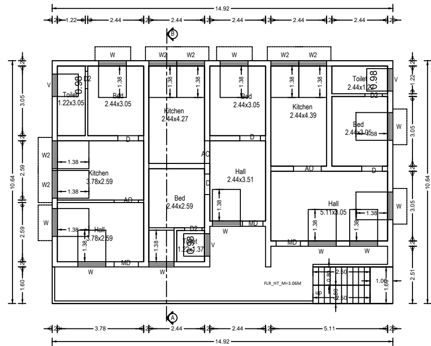
Plan Scale 1:100 Ground floor
