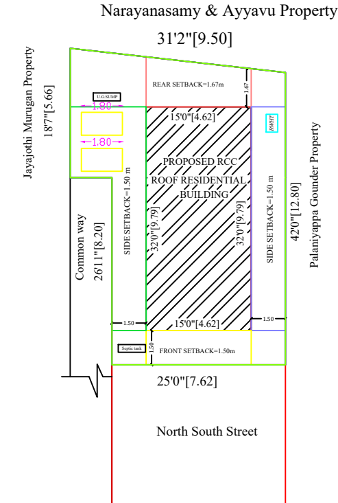
SITE PLAN
