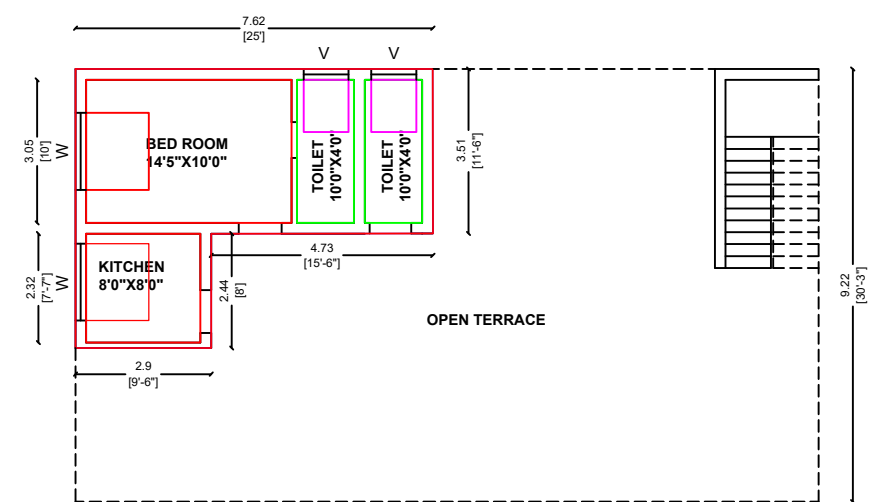
PROPOSED SECOND FLOOR
