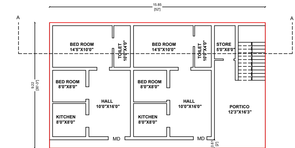
EXISTING GROUND FLOOR
