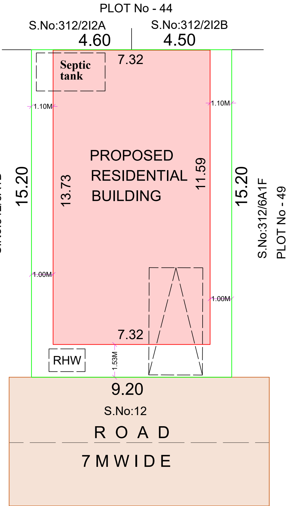
SITE PLAN
