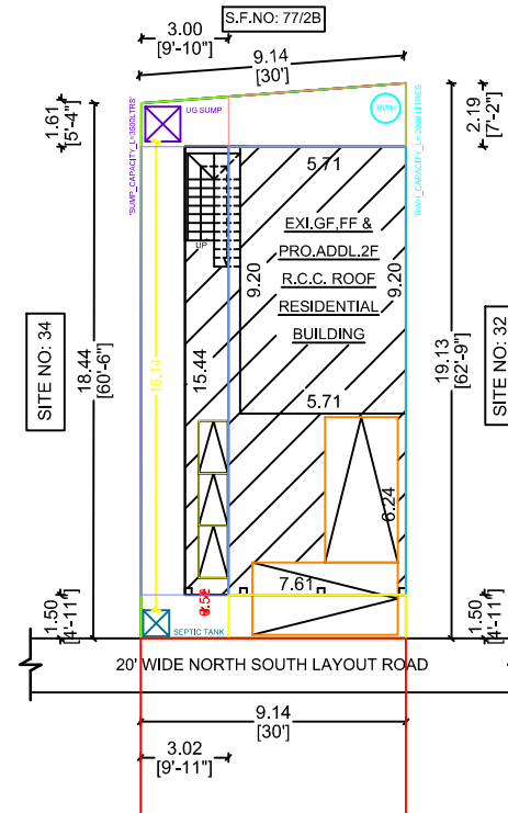
SITE PLAN
