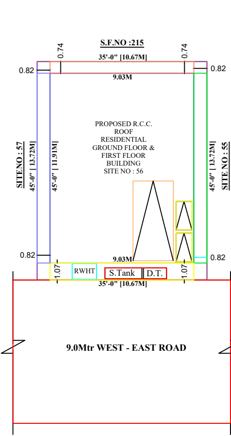
SITE PLAN
