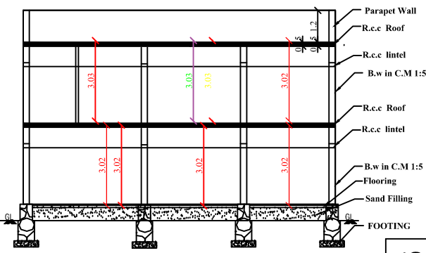
SECTION AB
