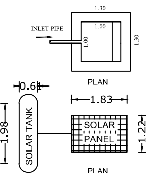
SOLAR SYSTEM
