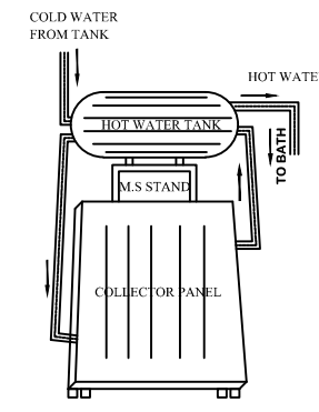
SOLAR WATER HEATER SYSTEM
