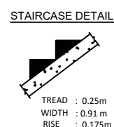
STAIRCASE DETAIL
