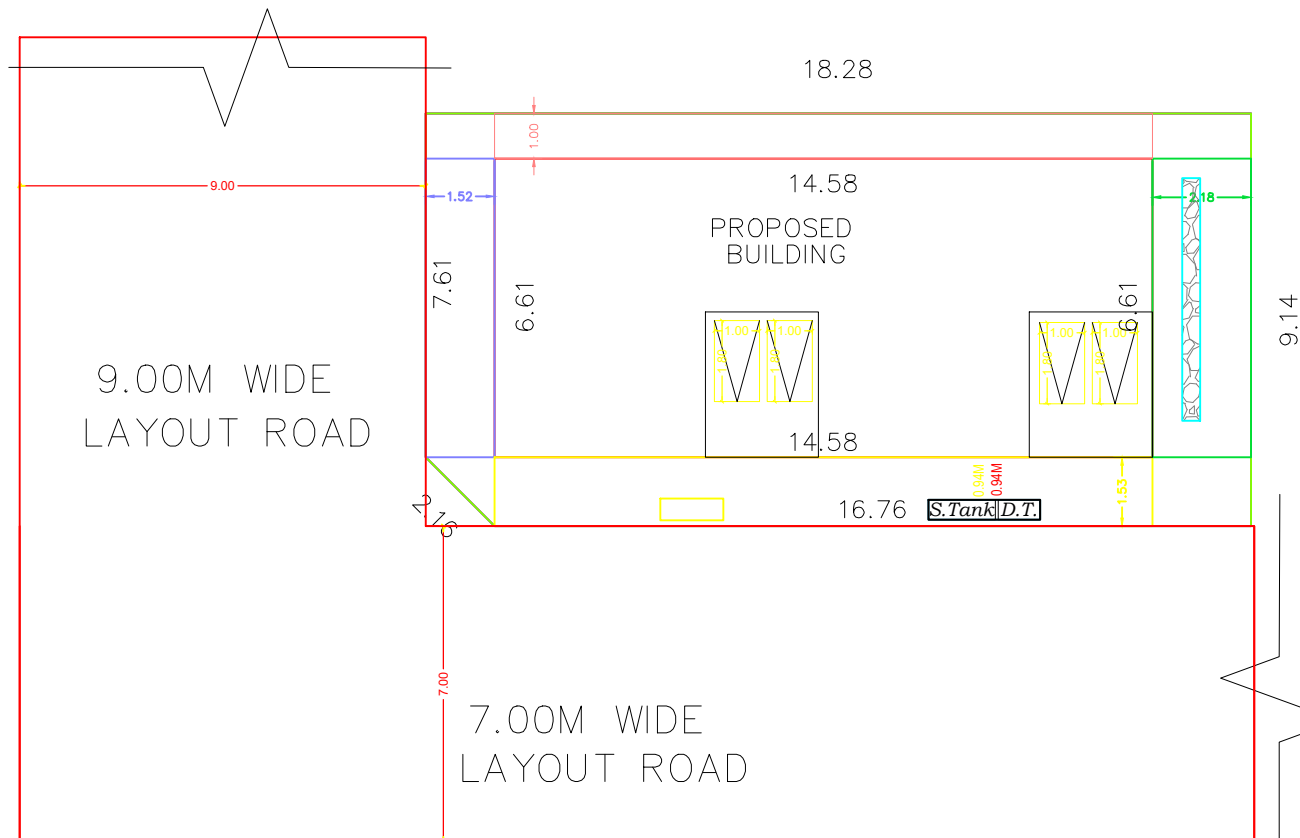
SITE PLAN
