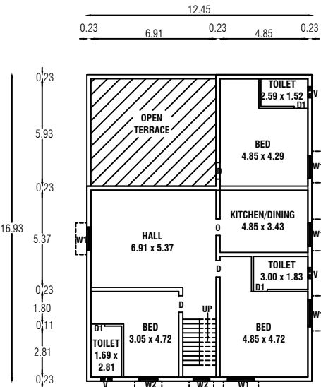
PROPOSED THIRD FLOOR PLAN
