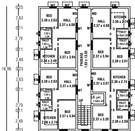
REVISED FIRST FLOOR PLAN
