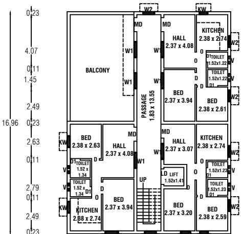
REVISED SECOND FLOOR PLAN
