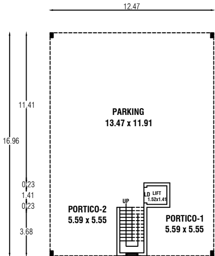
REVISED GROUND FLOOR PLAN
