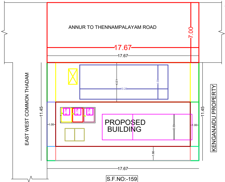
SITE PLAN
