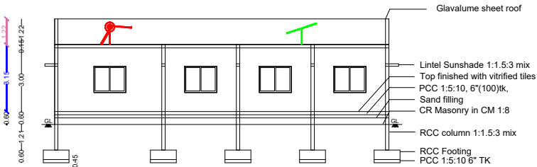
SECTION ON -'AA'
