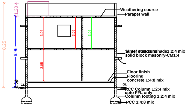
SECTION ELEVATION
