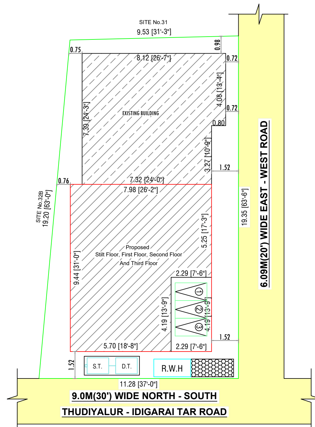
SITE PLAN
