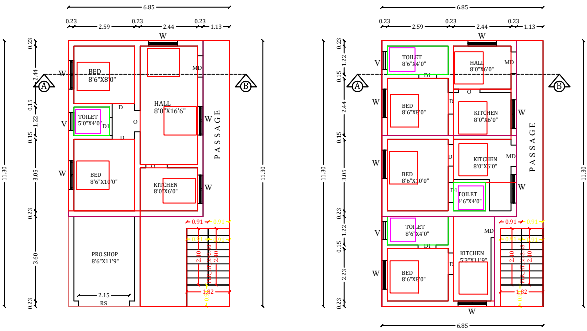
ALTERATION OF GROUND FLOOR PLAN
