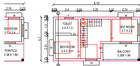
PROPOSED FIRST FLOOR PLAN
