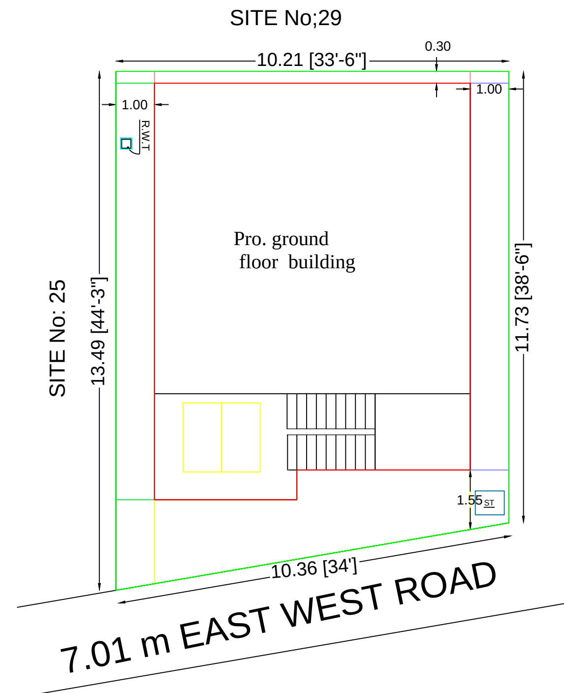
SITE PLAN
