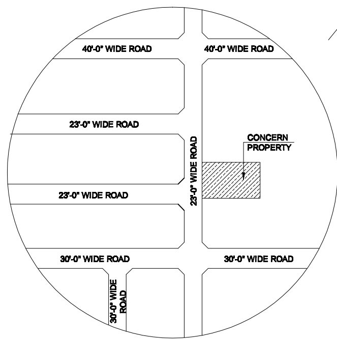
KEY PLAN
