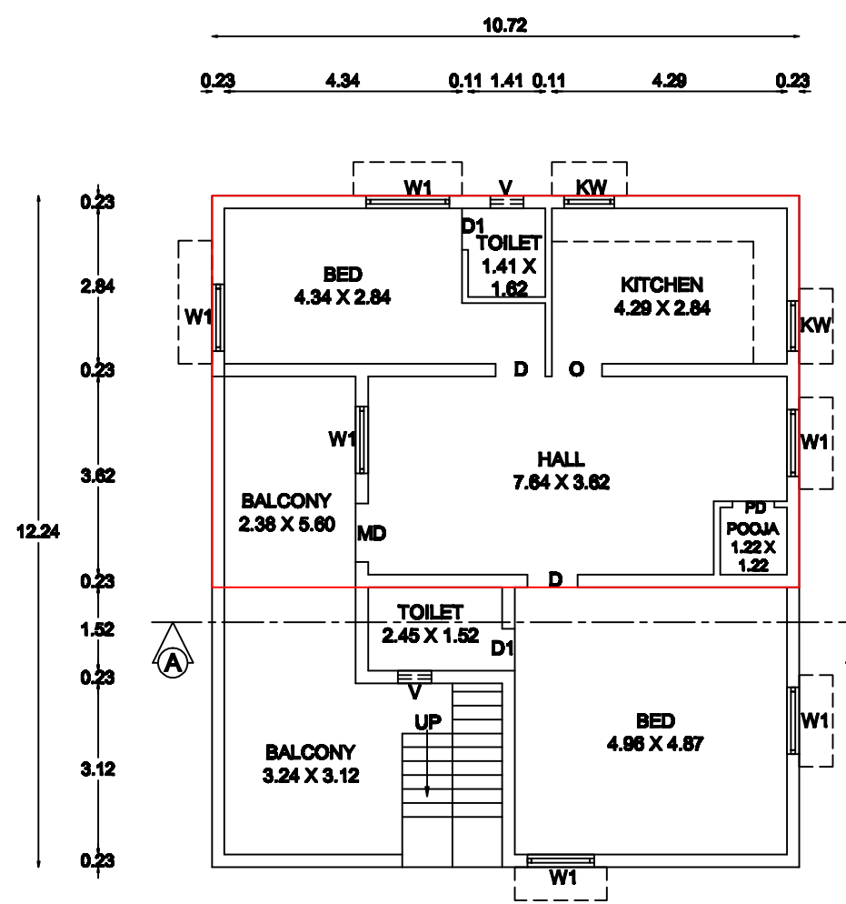
EXISTING FIRST FLOOR AND PROPOSED FIRST FLOOR PLAN
