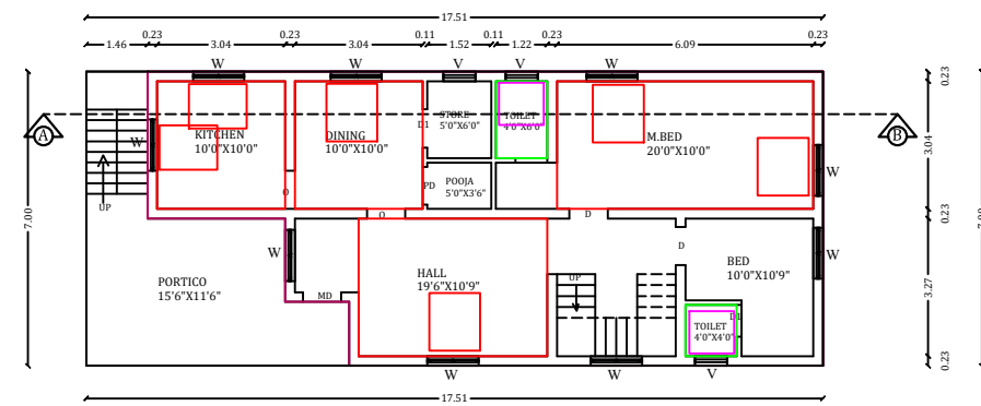
ALTERATION OF EXISTING GROUND FLOOR PLAN
