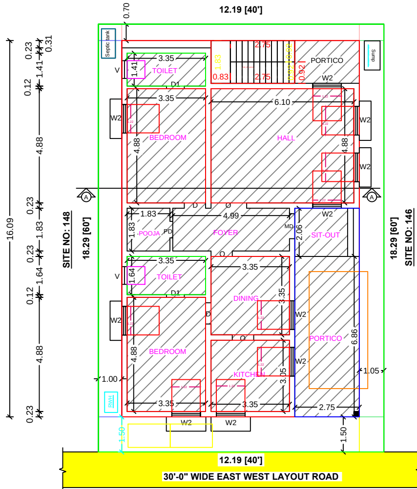
SITE CUM EXI.GROUND FLOOR PLAN
