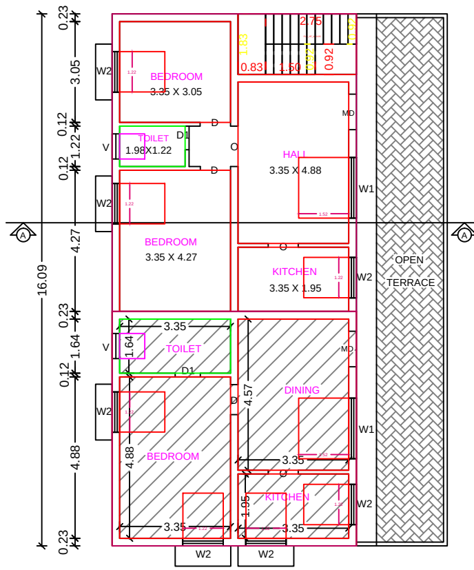
EXI. & ADD. PRO FIRST FLOOR PLAN
