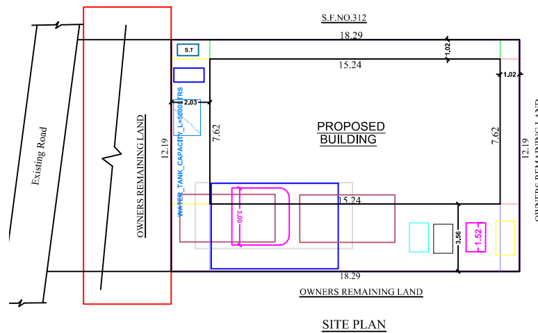
SITE PLAN
