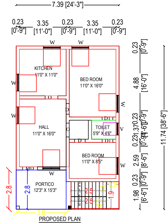
PROPOSED PLAN
