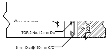
Typical Details of Providing Vertical Steel Bars Around Door / Windows
