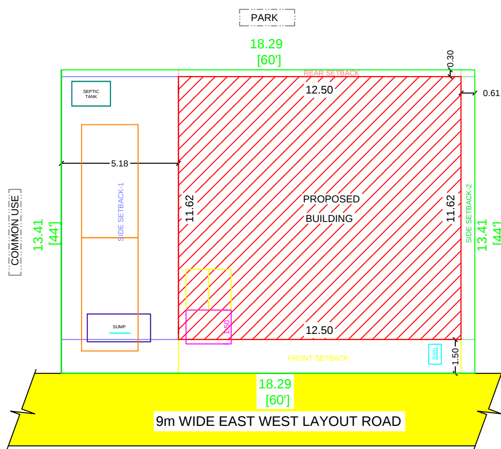
SITE PLAN
