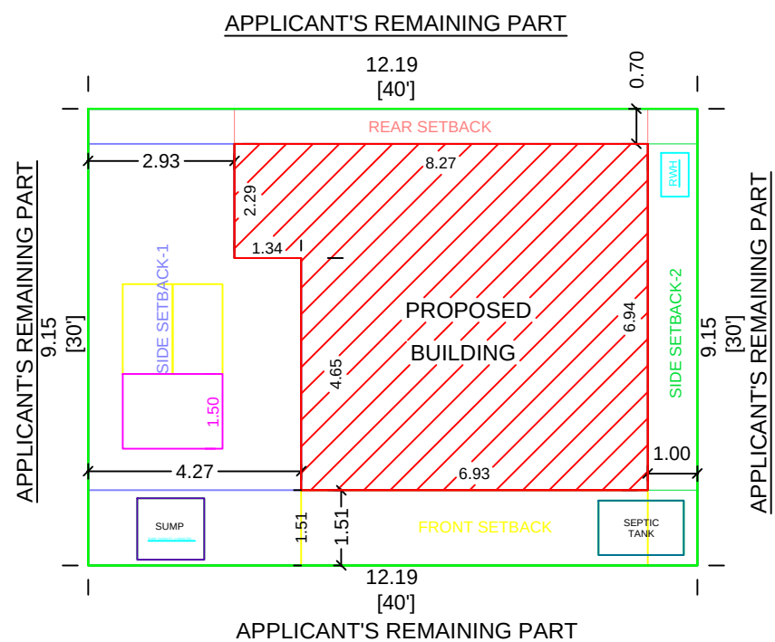
SITE PLAN
