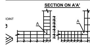
SECTION ON 'A-A'
