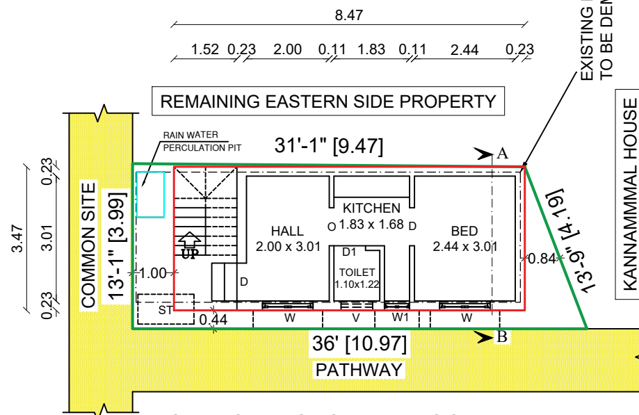
SITE CUM GROUND FLOOR PLAN
