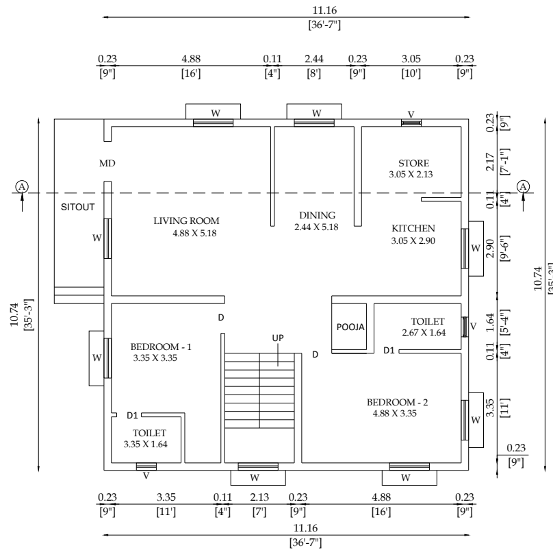
GROUND FLOOR BUILDING PLAN
