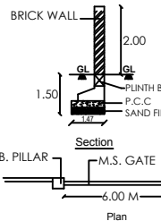
Compound Wall & Gate Details
