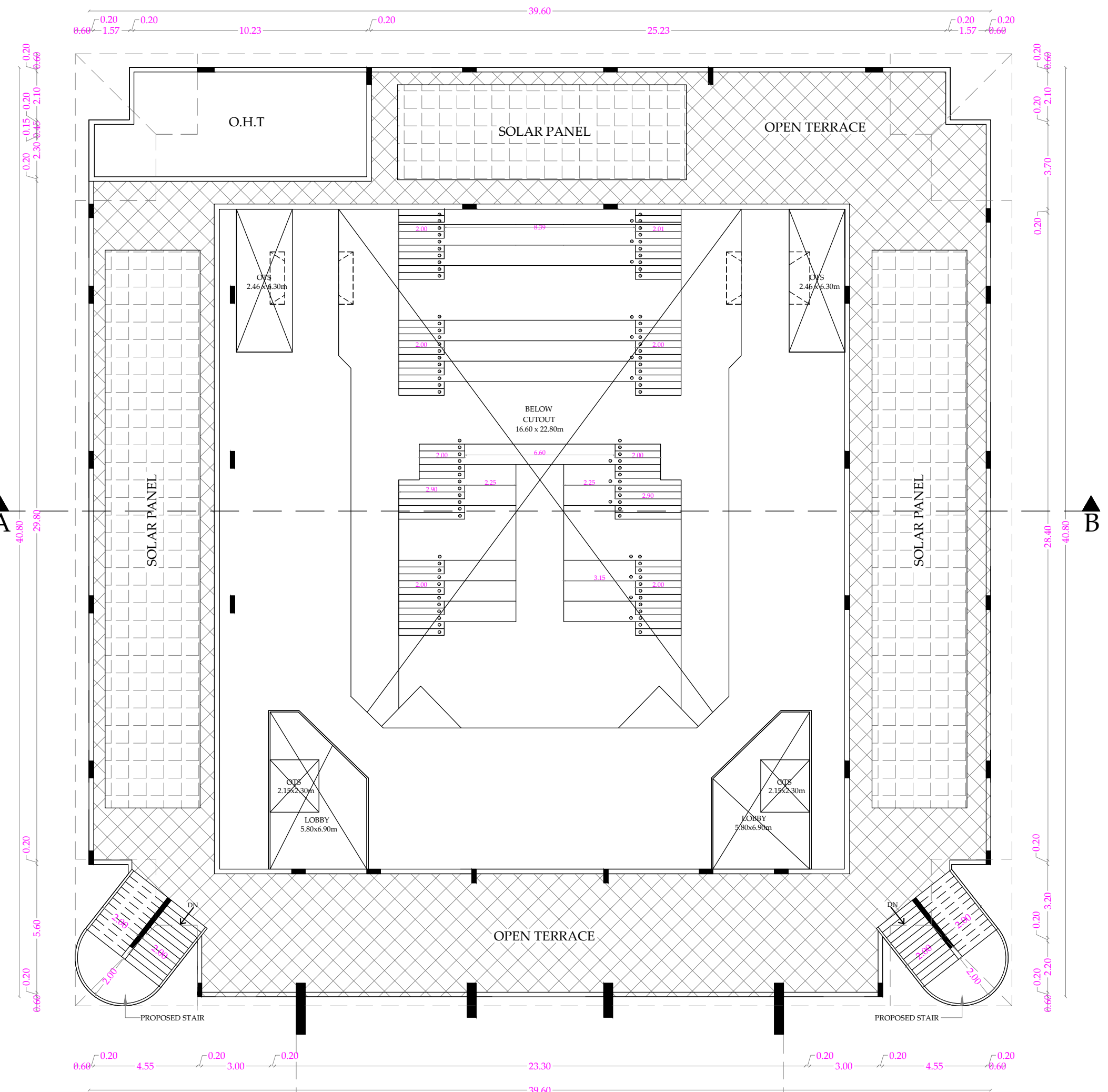
ADDITIONAL TERRACE FLOOR PLAN
