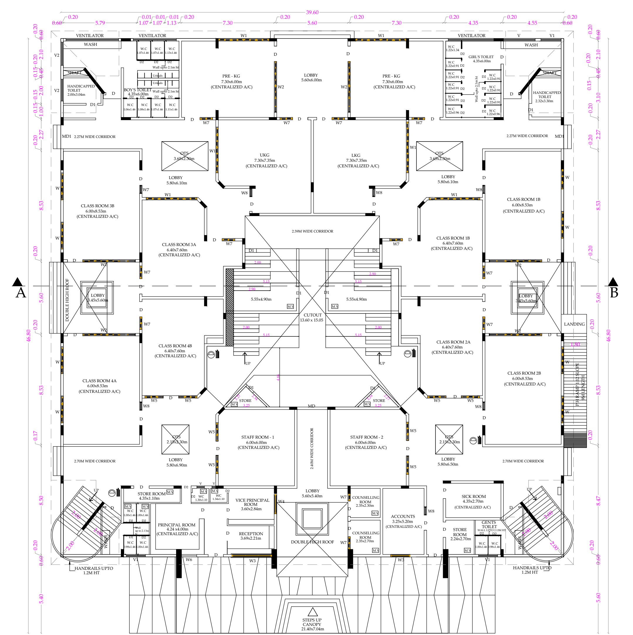
REVISED GROUND FLOOR PLAN
