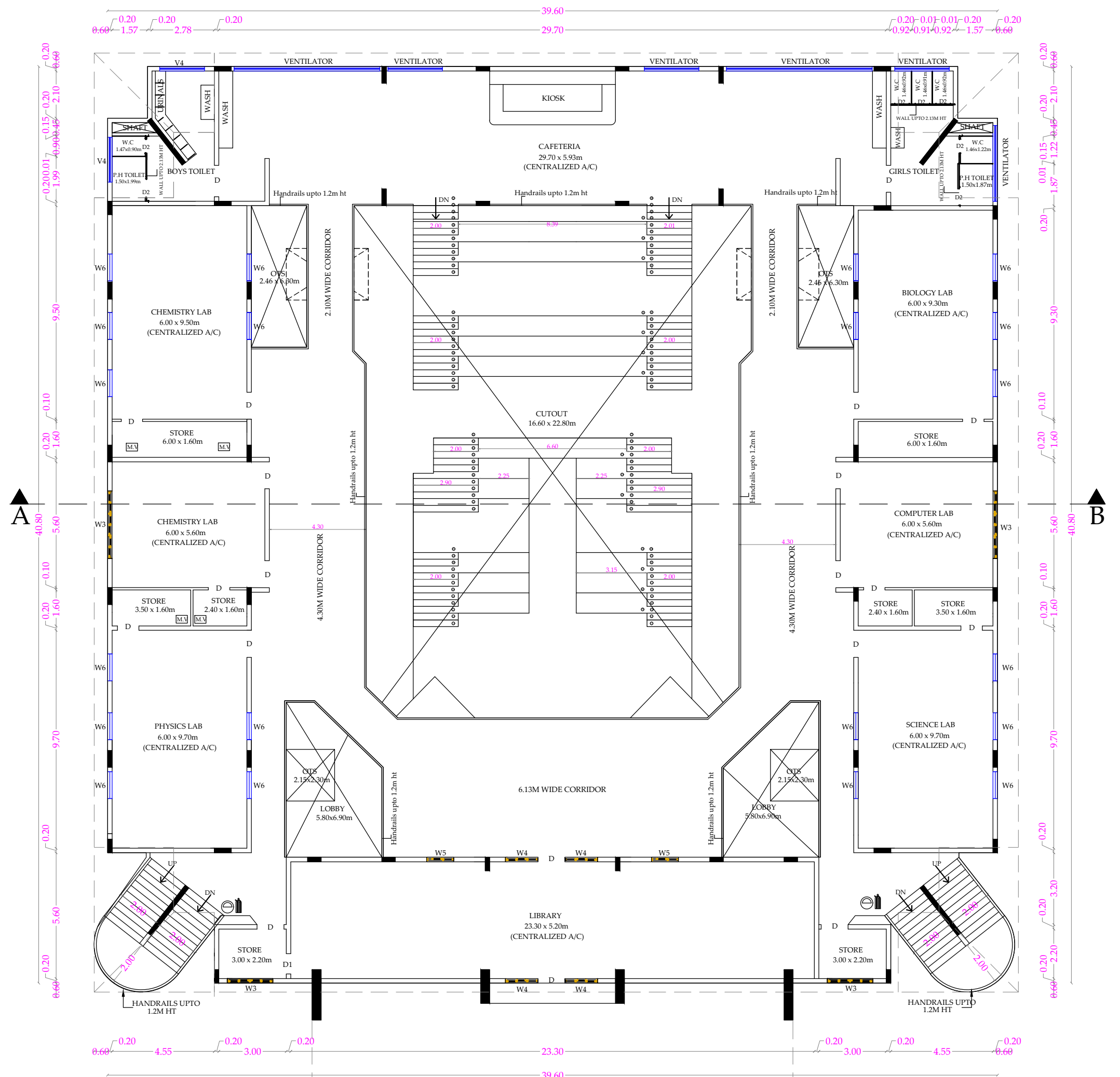
ADDITIONAL SECOND FLOOR PLAN
