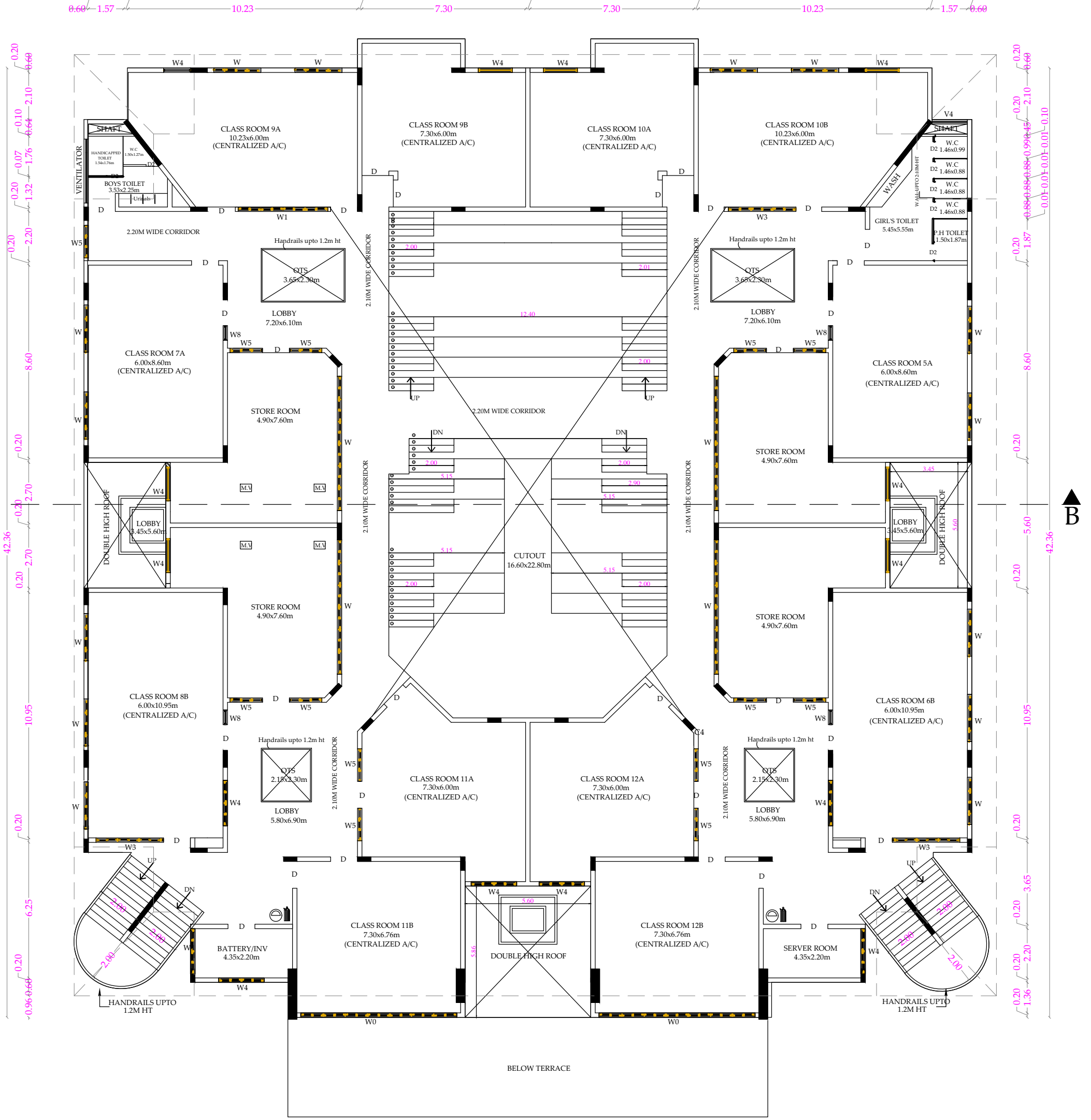
REVISED FIRST FLOOR PLAN
