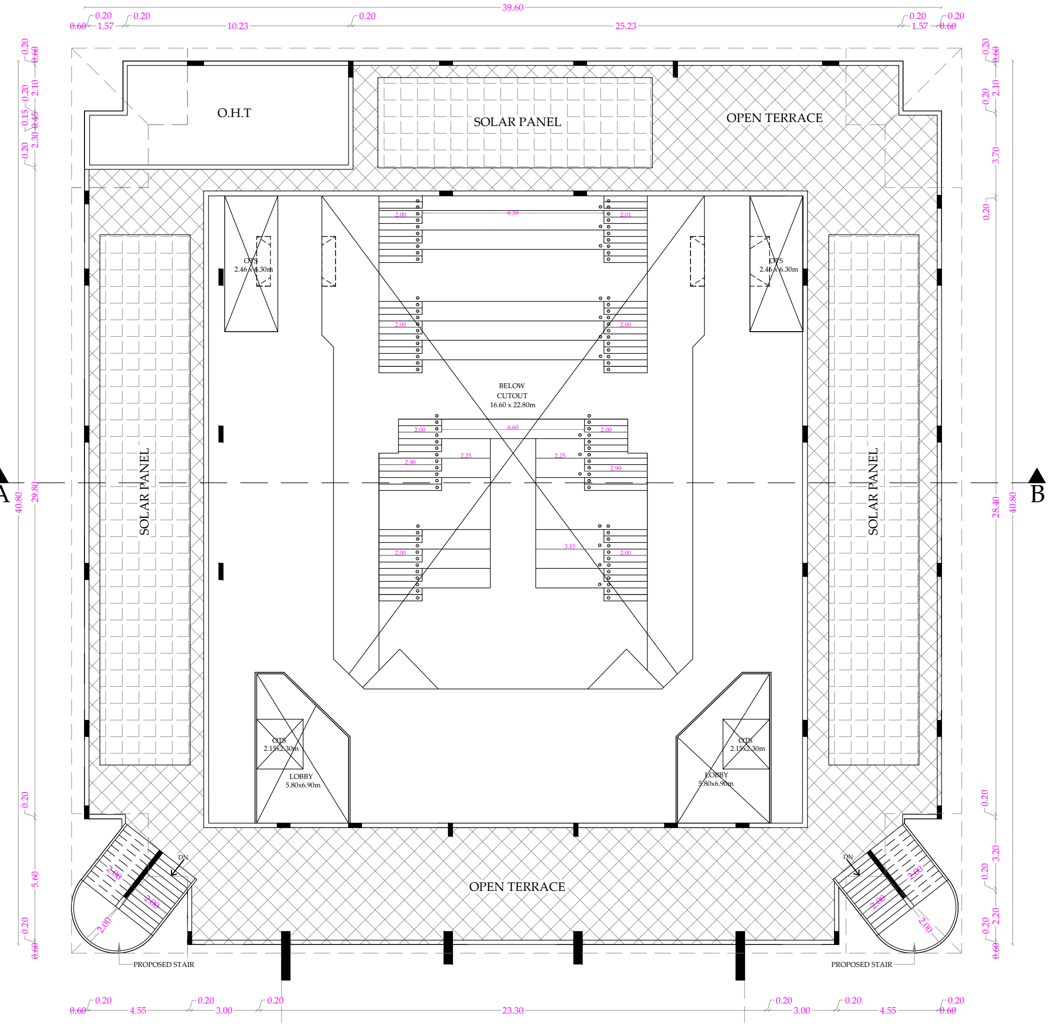
ADDITIONAL TERRACE FLOOR PLAN
