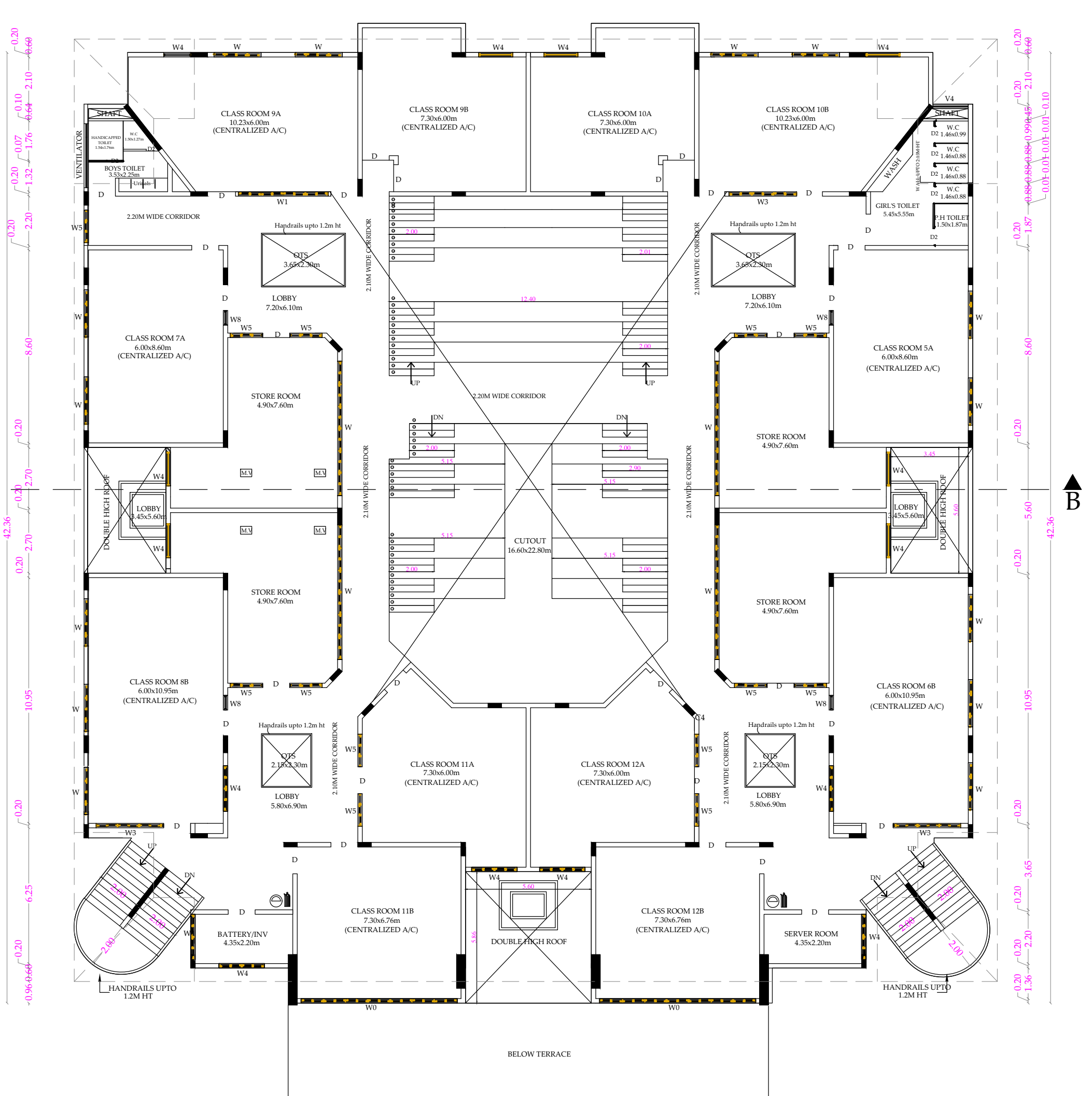
REVISED FIRST FLOOR PLAN
