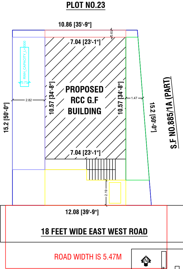
SITE PLAN
