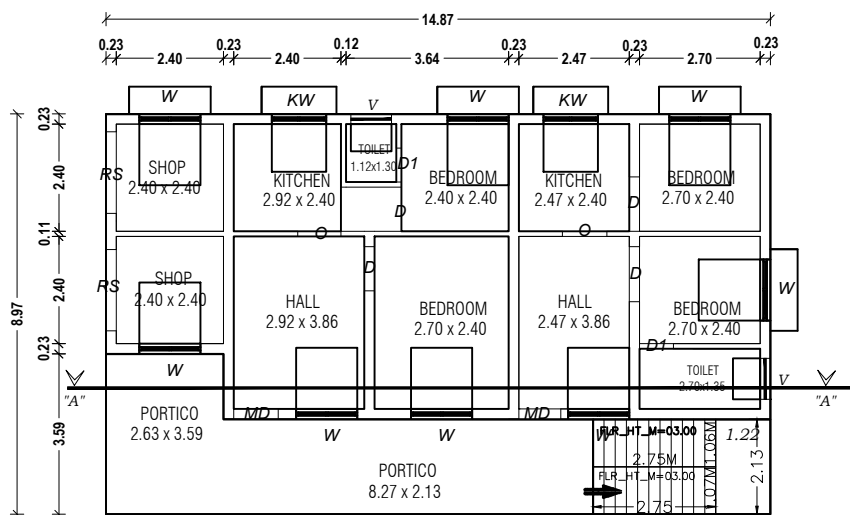
EX. GROUND FLOOR PLAN
