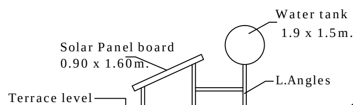
CROSS SECTION OF SOLAR WATER HEATING SYSTEM
