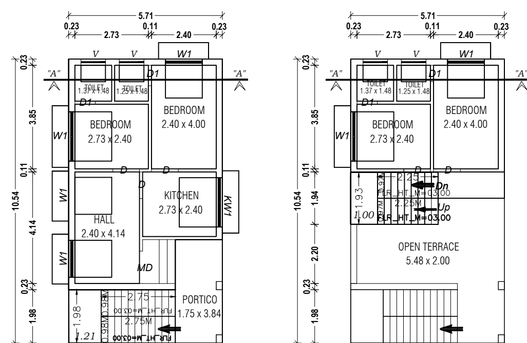
FLOOR PLAN PRO-FIRST FLOOR PLAN
