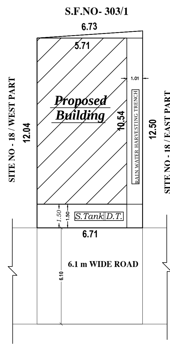
SITE PLAN
