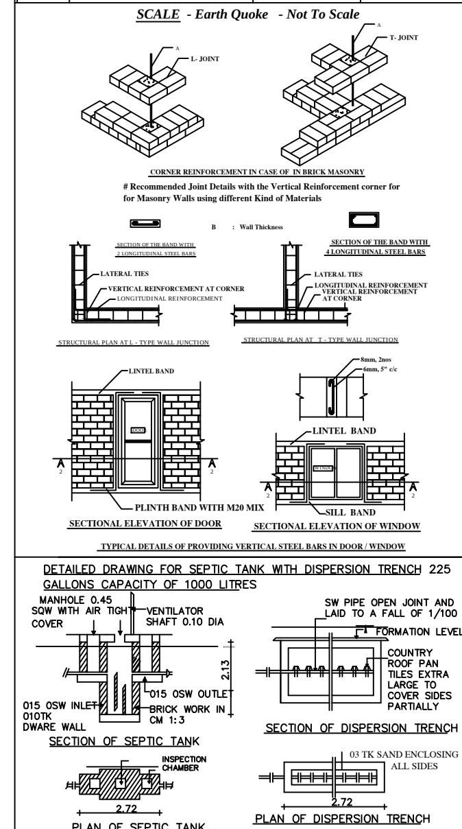
DETAILED DRAWING FOR SEPTIC TANK WITH DISPERSION TRENCH 225 GALLONS CAPACITY OF 1000 LITRES
