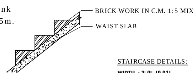
STAIRCASE DETAILS (NOT TO SCALE)
