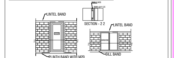
FIGURE 2: REINFORCEMENT AND BENDING DETAILS OF SEISMIC BANDS
