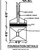
FOUNDATION DETAILS (NOT TO SCALE)
