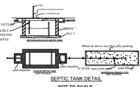
SEPTIC TANK DETAIL (NOT TO SCALE)
