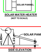
SOLAR PANNEL SOLAR WATER HEATER (NOT TO SCALE)
