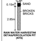
RAIN WATER HARVESTING DETAIL PERCOLATION PIT (NTS)
