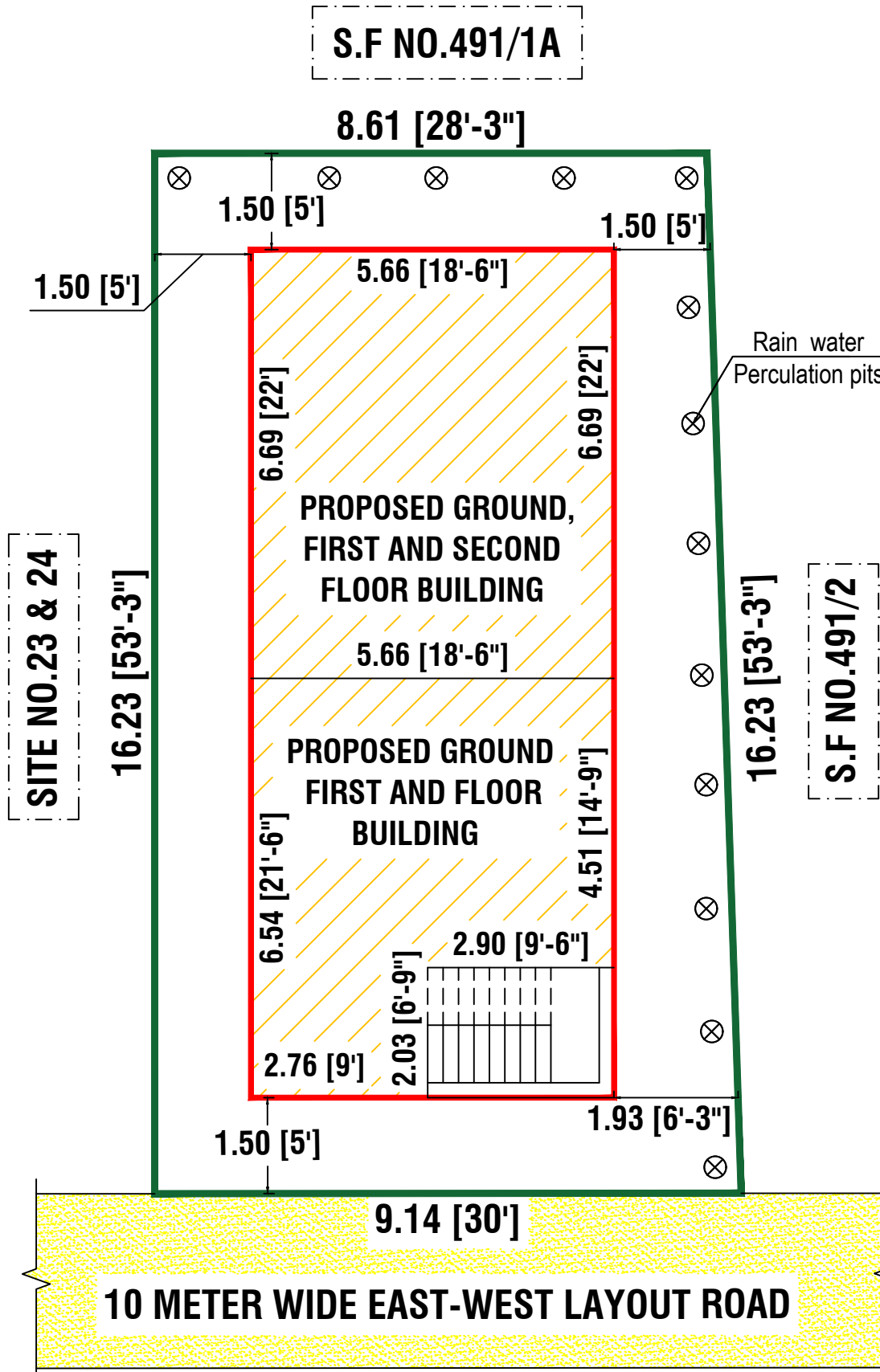
SITE PLAN
