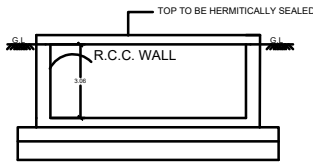
RWH SECTION (SAMPLE)
