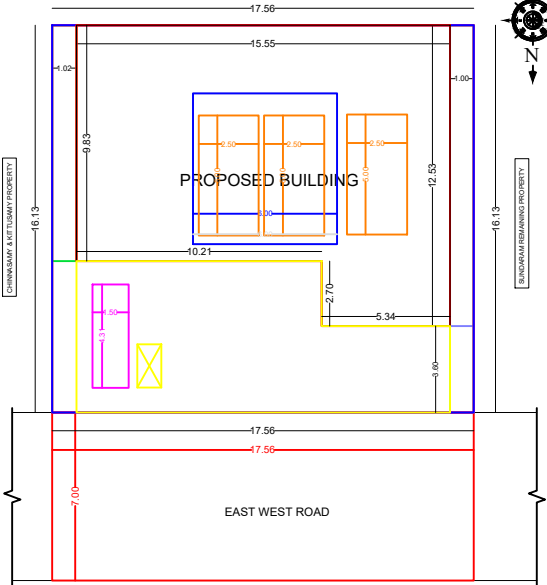
SITE PLAN
