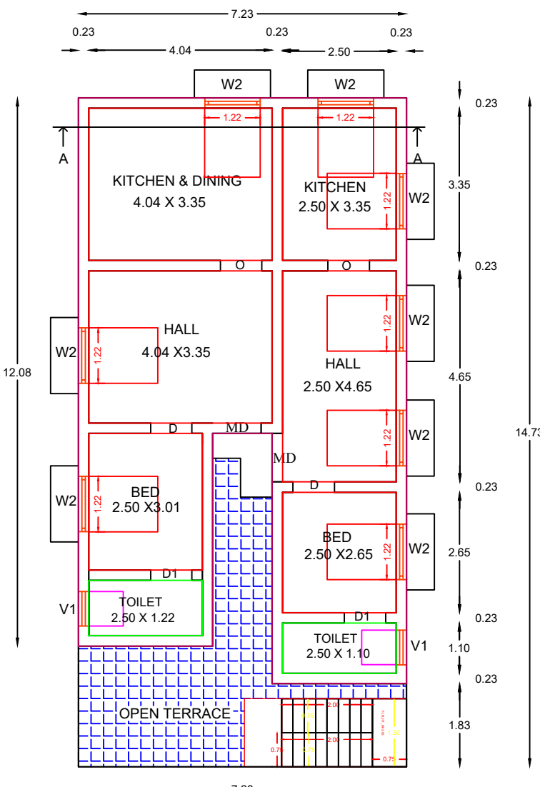
PRO.ADDL SECOND FLOOR PLAN
