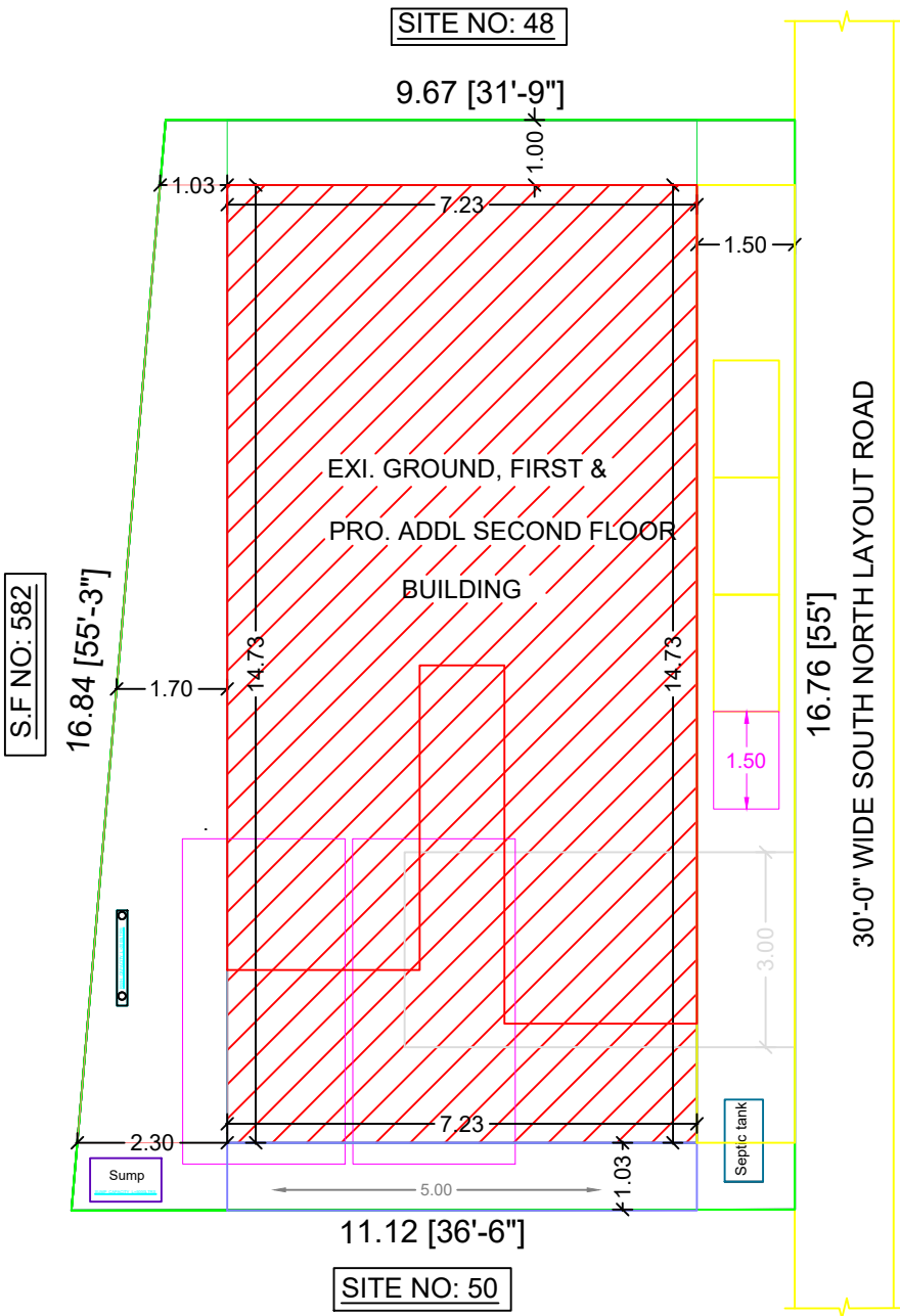
SITE PLAN
