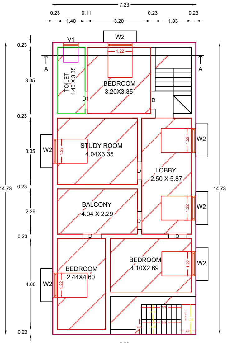
EXI.FIRST FLOOR PLAN
